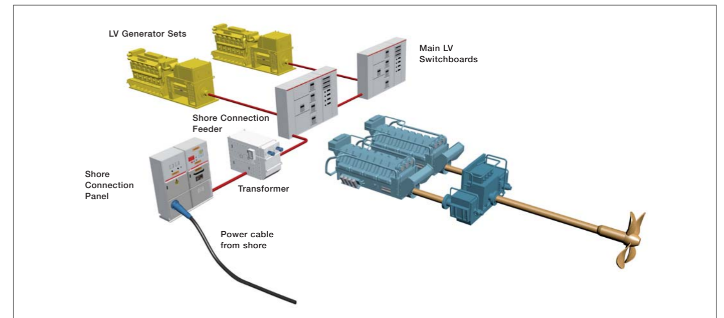
Figure 2 shows a ship with diesel machinery and low voltage electric system. The Shore Connection System is arranged with the Shore Connection Panel located outside the main switchboard room with cable connectors mounted in the front. An onboard transformer steps down the power from high to low voltage.
