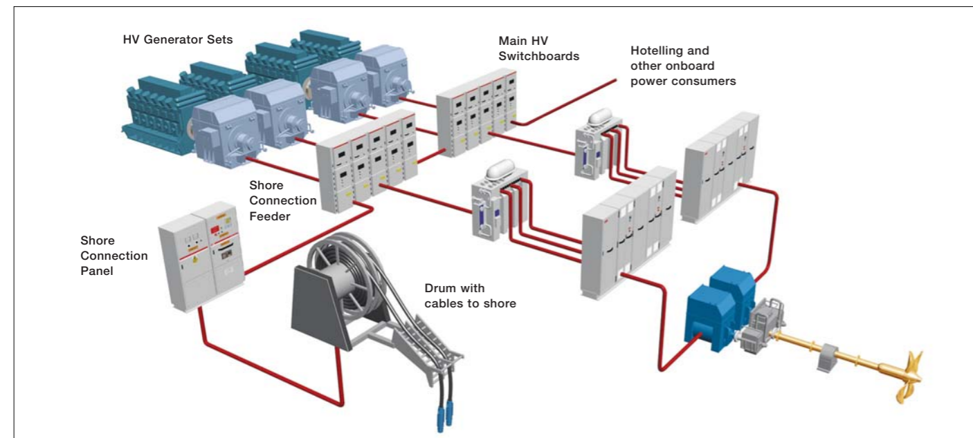
Figure 1 shows a ship with diesel-electric propulsion and a Shore Connection system configured with the Shore Connection Panel located outside the main switchboard room. The ship is equipped with an onboard cable drum to lower the cable down to the quay for onshore termination.
