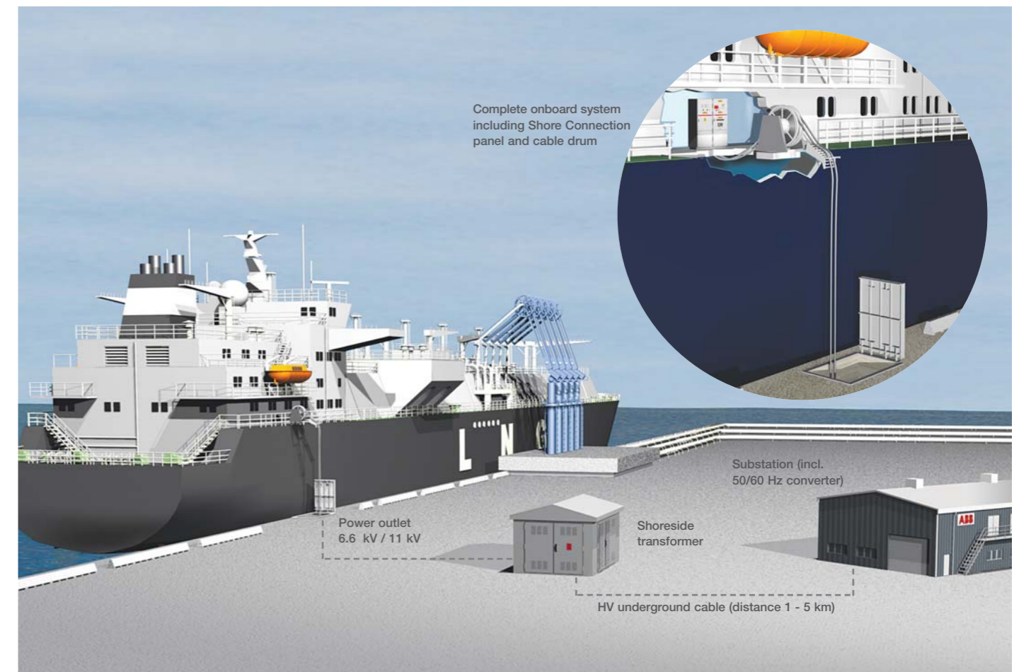
ABB Shore Connection is a modular and highly flexible system that can be adapted to the unique requirements of each project. The system is easy to implement onboard and the shoreside equipment - transformer and substation - is built in modules for both small and large ports.
