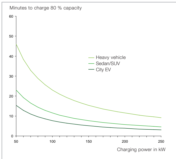
Charging speed
